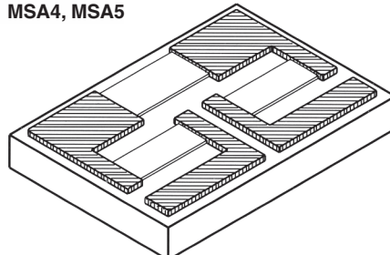
MSA4, MSA5
