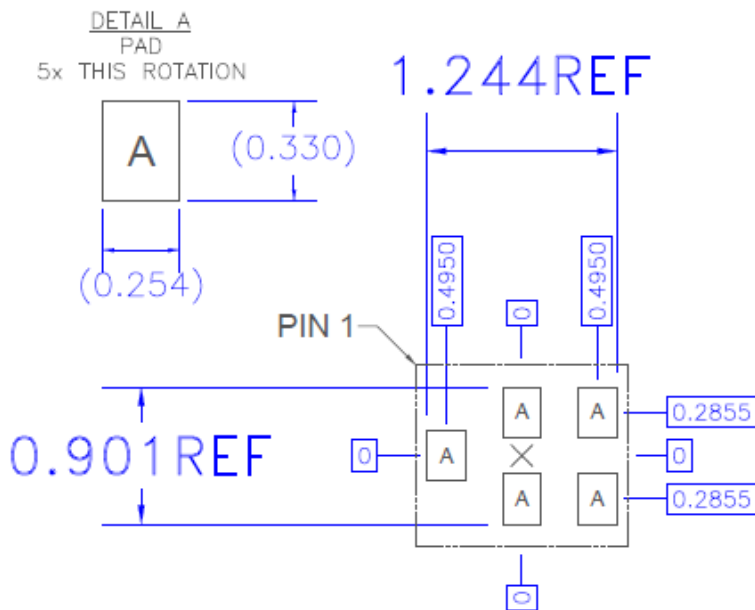
Reocmmended Landing Pattern
