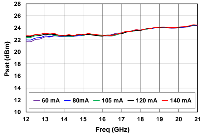
Psat vs Current
