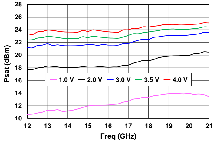
Psat vs Voltage
