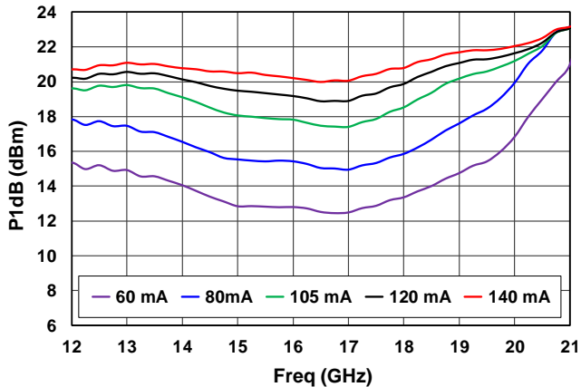
P1dB vs Current
