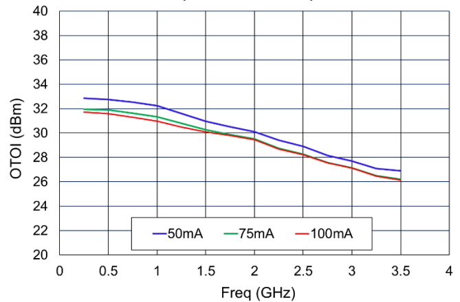
Output TOI vs Freq vs Ids
