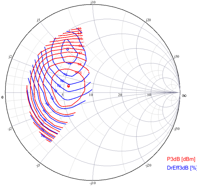
Load Pull at 2.1 GHz
