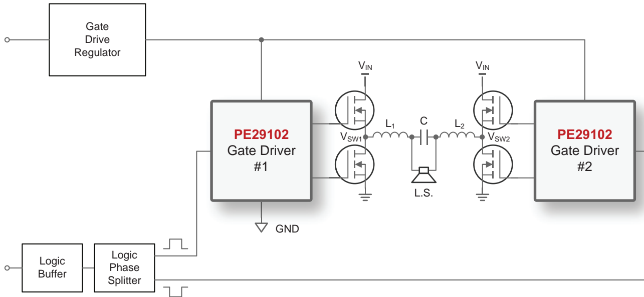
Figure 8 ■ PE29102 Class D Audio Amplifier Block Diagram
