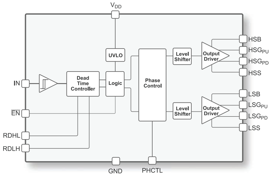
Figure 1 ■ PE29102 Functional Diagram
